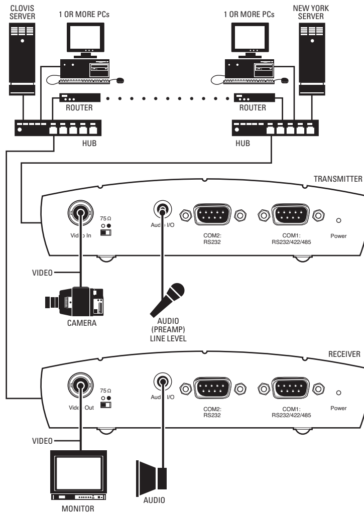
Figure 10. WAN Box-To-Box Connection (Transmitter, Receiver, Fixed Camera)
